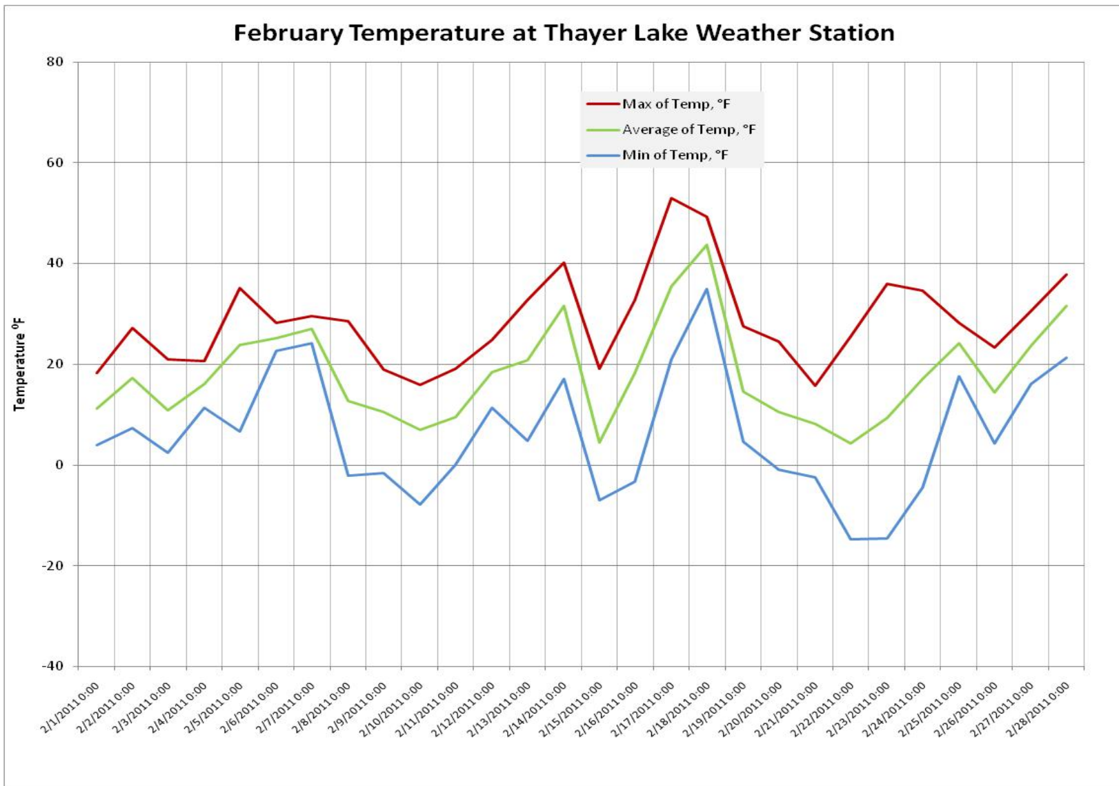
Figure 4: Thayer Lake Weather Station February 2011 mean, maximum and minimum temperature in degrees Fahrenheit.
