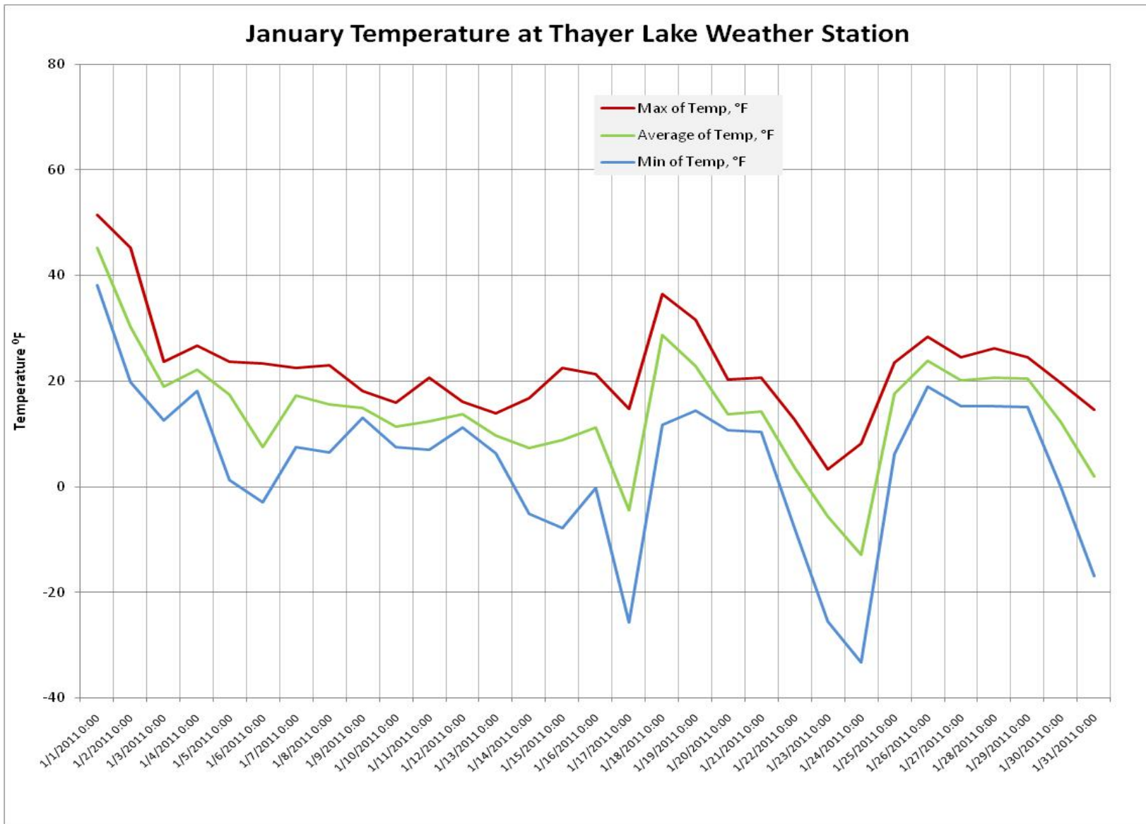
Figure 3: Thayer Lake Weather Station January, 2011 mean, maximum and minimum temperature in degrees Fahrenheit.
