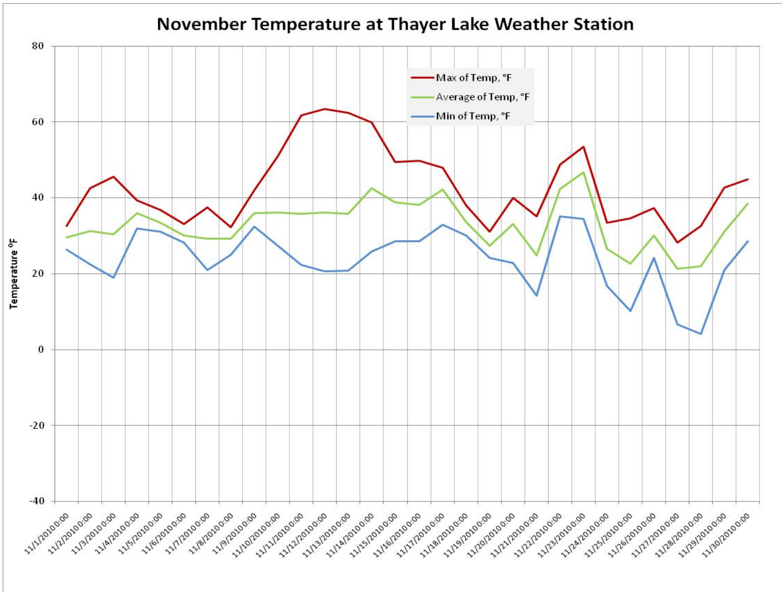
Figure 1: Thayer Lake Weather Station November 2010 mean, maximum and minimum temperature in degrees Fahrenheit.
