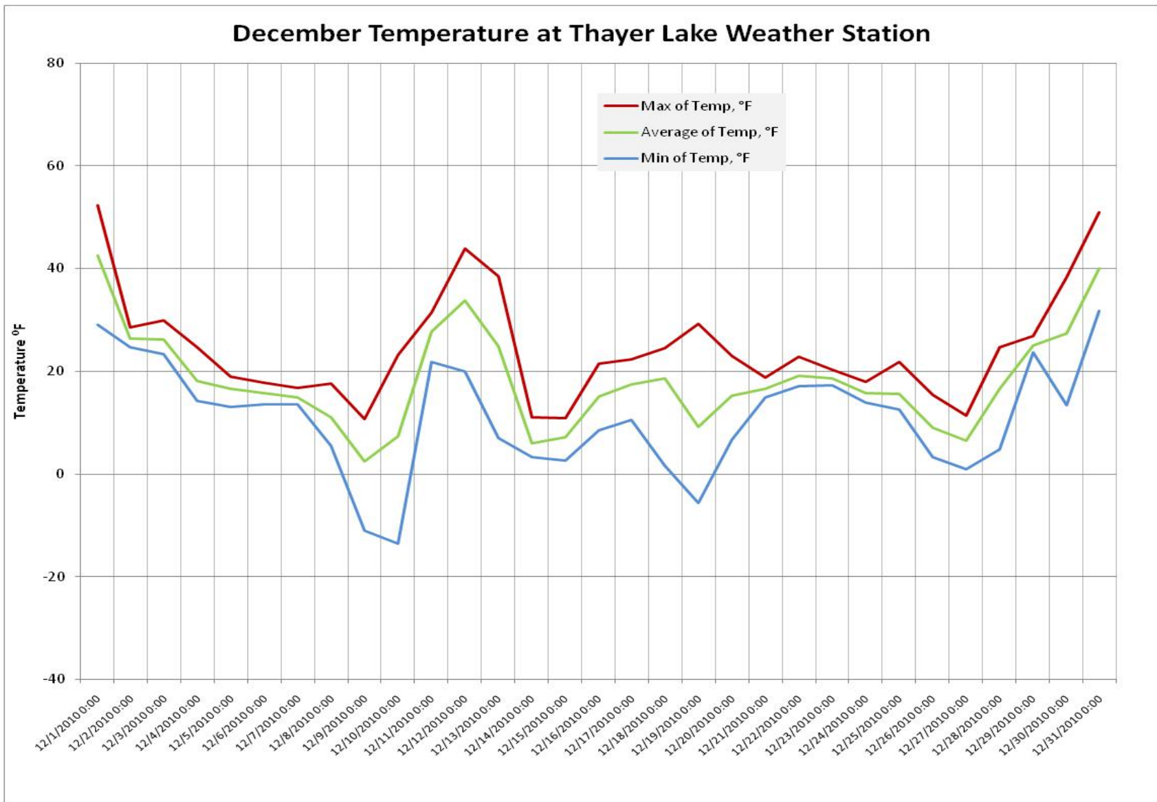
Figure 2: Thayer Lake Weather Station December 2010 mean, maximum and minimum temperature in degrees Fahrenheit.
